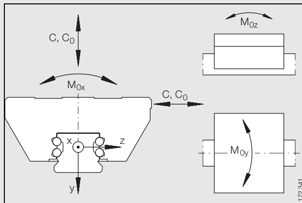
Load direction
